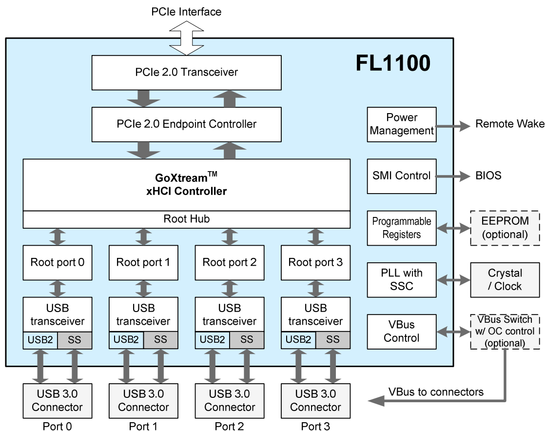
Figure 3-1 FL1100 block diagram
