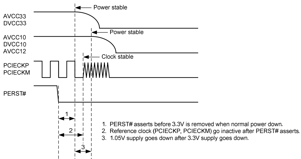
Figure 4-2 Power-down Sequence
