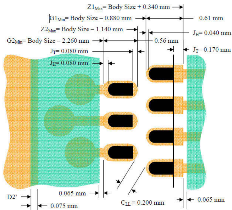
Figure 4 Land pattern of PCB for 0.5mm pitch DRQFN
