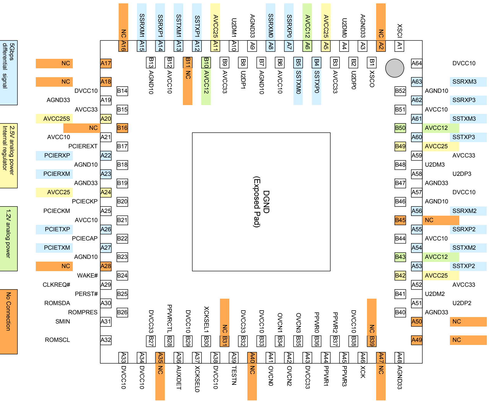
Figure 2-1 shows the ballout map of FL1100 from the top of the package view.
