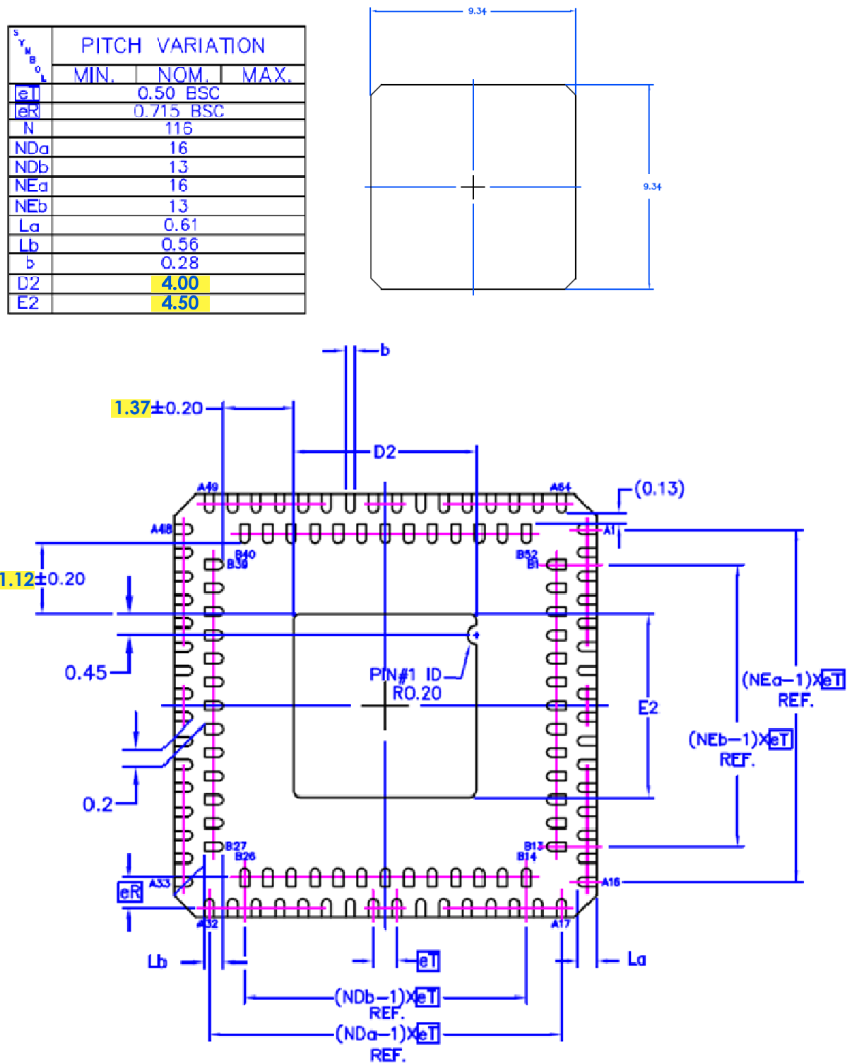
Figure 5 PCB footprint of DRQFN
